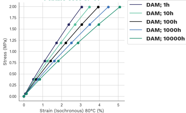
Stress-strain (Isochronous) 80°C Pebax® 5533 SP 01
